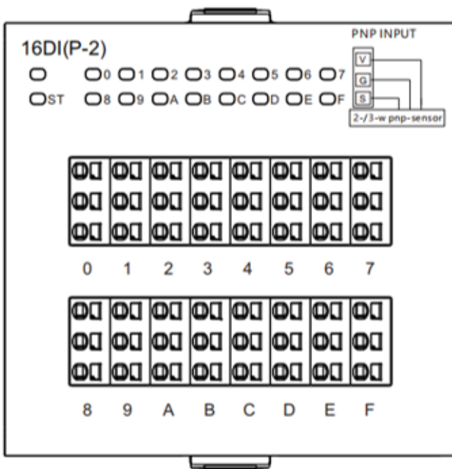
16DI(P-2)
