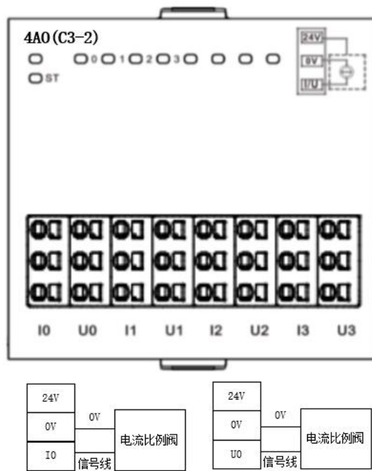
4AO(C3-2)
