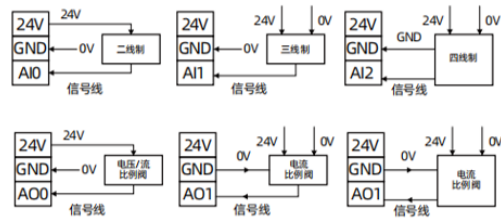
4AI2AO(I5-2)
