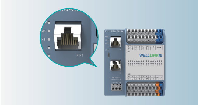
The communication interface port is designed to be inclined to 45 degrees
